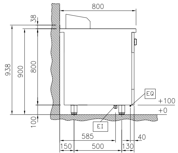
Lateral
